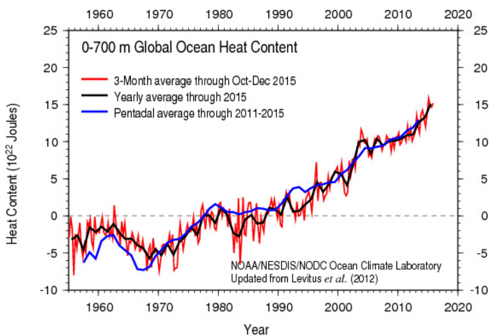
Figure 1: Ocean heat content down to a depth of 700 m: 3-month averages (red), 5-year averages (blue), and annual averages (black). Source: NOAA National Centers for Environmental Information 2015a.
